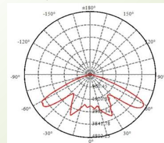
R2 Diagram for luminous intensity distribution
