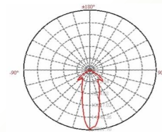
R1 Diagram for luminous intensity distribution
